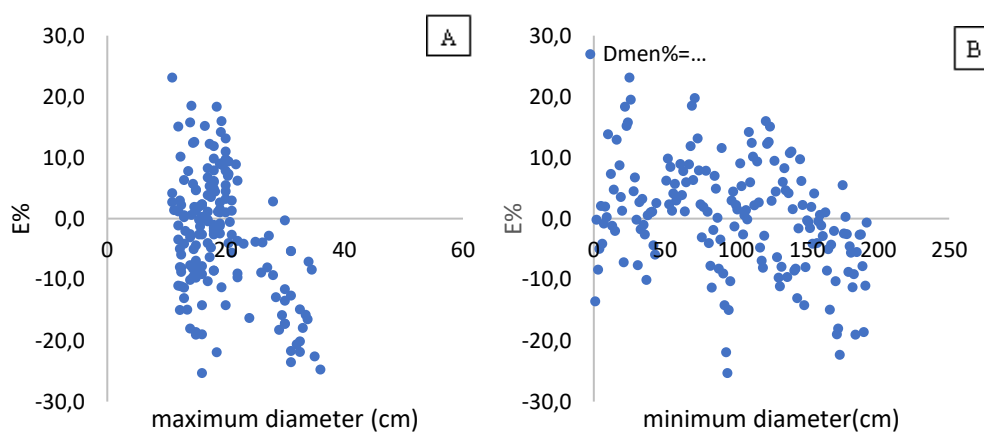
Figure 6: (A) E% as a function of the maximum diameter, and (B) E% as a function of the minimum diameter of the part in Test 2
