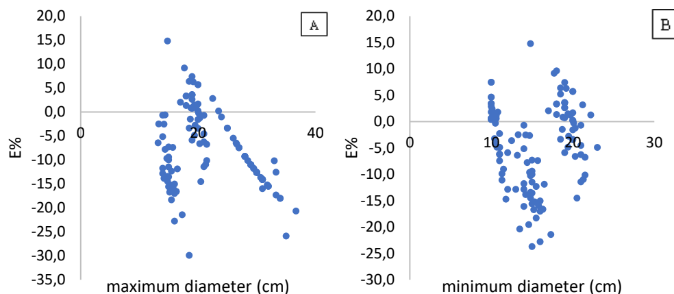
Figure 5: (A) E% as a function of the maximum diameter, and (B) E% as a function of the minimum diameter of the part in Test 1
