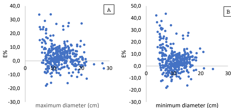
Figure 7: (a) E% as a function of the maximum diameter, and (b) E% as a function of the minimum diameter of the part in Test 3
